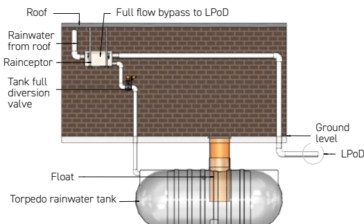
TYPICAL INSTALLATION
